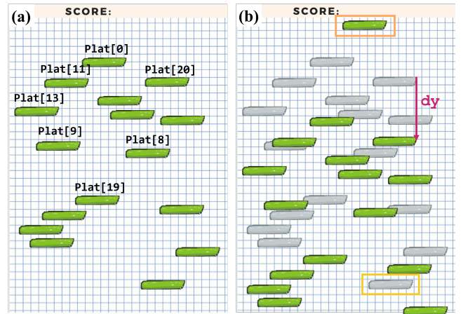
Fig. 3. Diagram to Show How Platforms are Initialized and Moved
